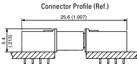
Example of combined receptacle and plug
